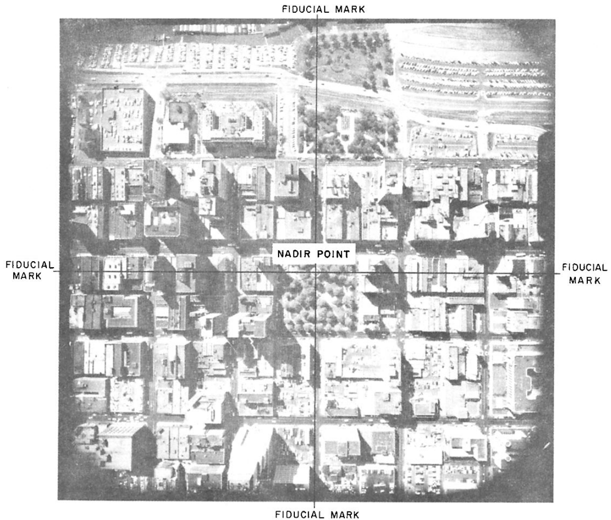
Figure 7-4.—Relief displacement.
